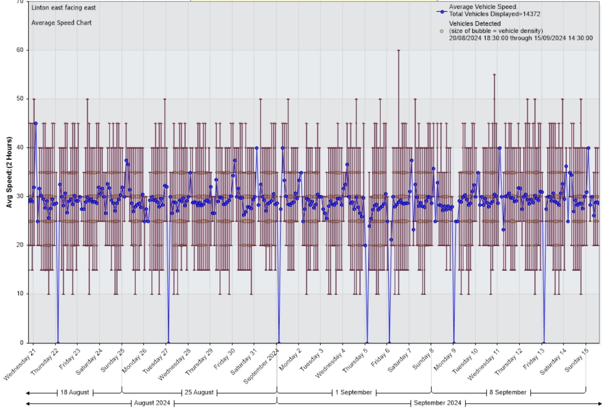
Average Vehicle Speed (MPH) vs. Time [Linton east facing east:Incoming]
