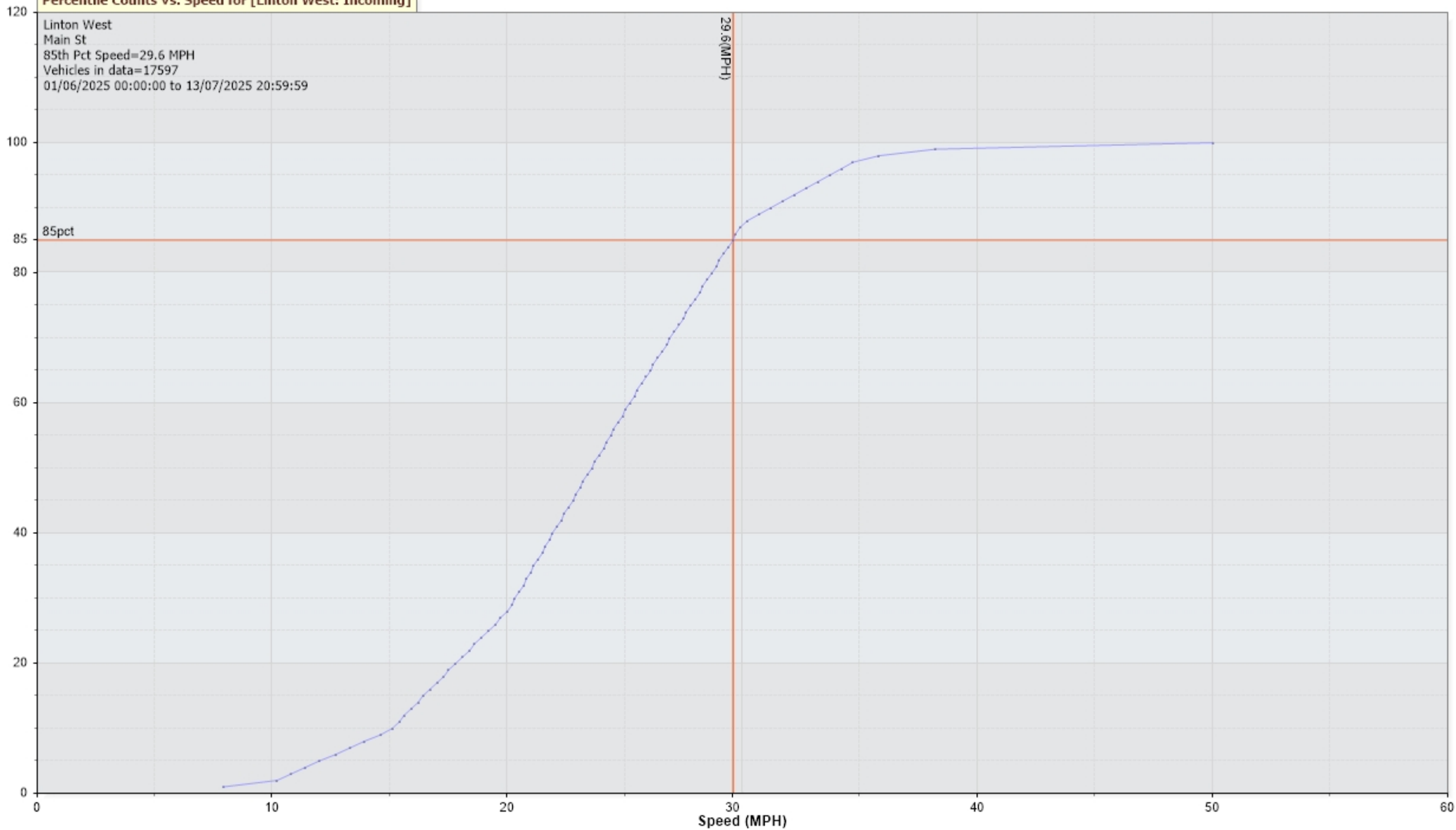
Percentile Counts Vs. Speed for [Linton West: Incoming]
